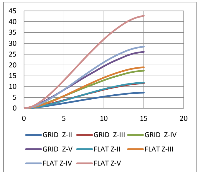
Graph 4– Storey Displacement (in cm) along Y-Direction
