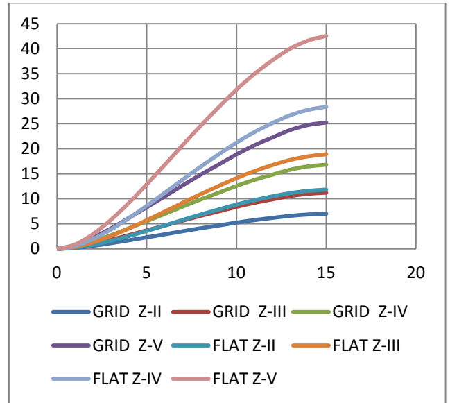
Graph 3– Storey Displacement (in cm) along X-Direction
