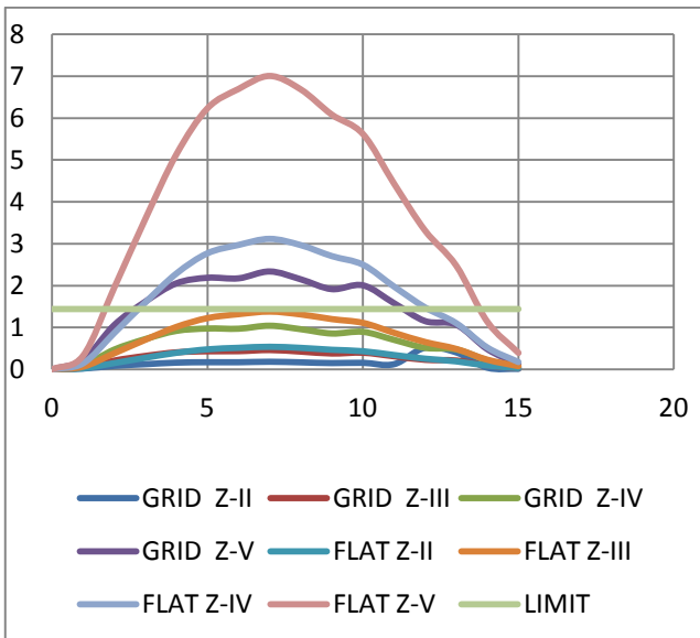
Graph 6– Storey Drift (in cm) along Y-Direction
