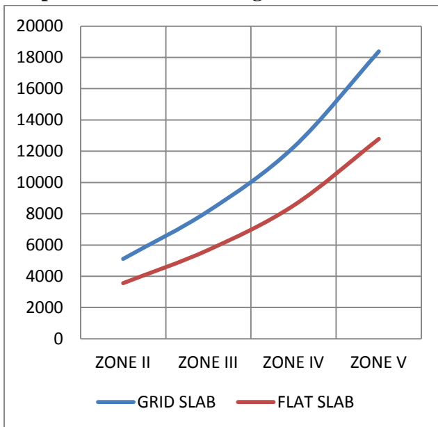
Graph 1– Base Shear along X-Direction
