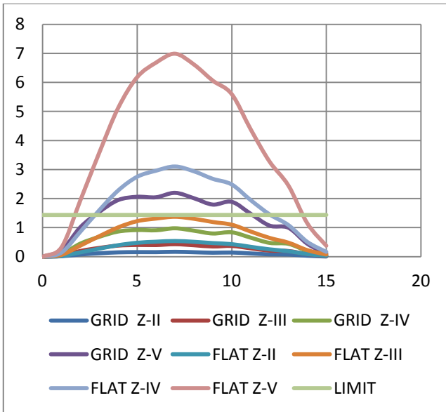
Graph 5– Storey Drift (in cm) along X-Direction
