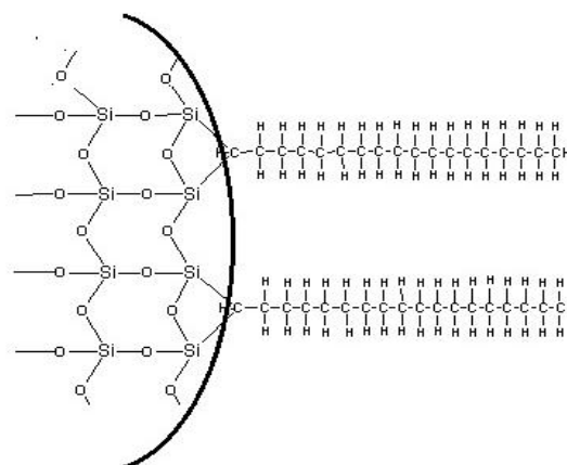
Fig. 03. C18 Column silica with bonded octadecyl alkyl chain
